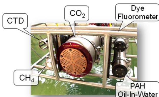
Underwater ROV Inspection Sensor System, application example with industrial high-grade sensors for Oil+Gas offshore surveys
